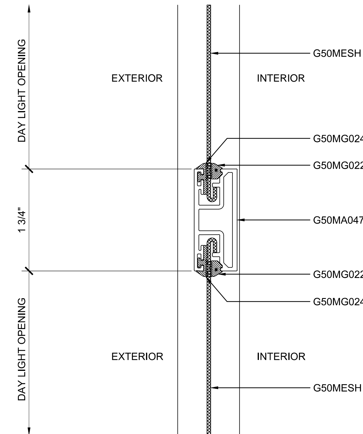
③ SECTION DETAIL AT MIDRAIL - OPTIONAL
