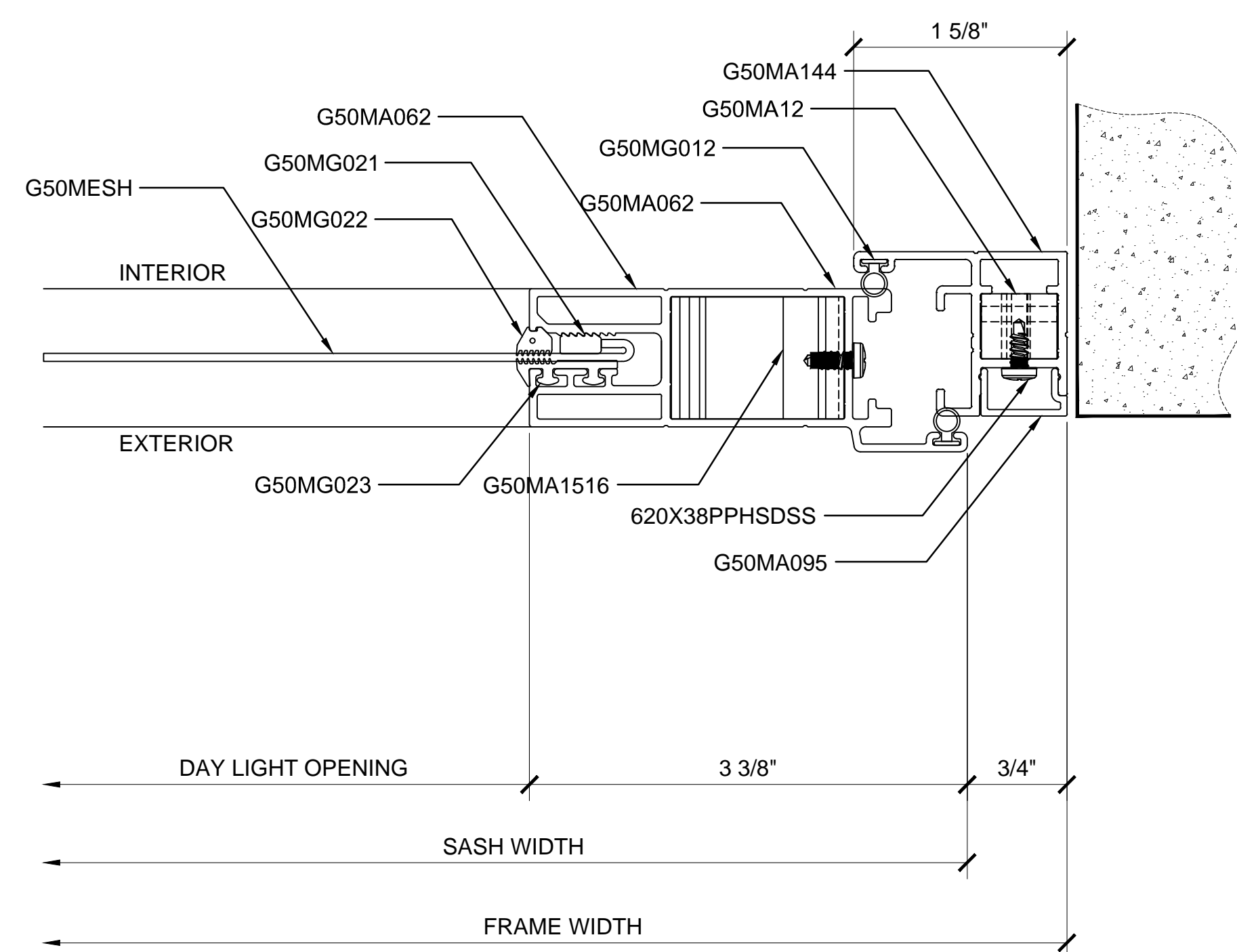
② SECTION DETAIL AT JAMB
