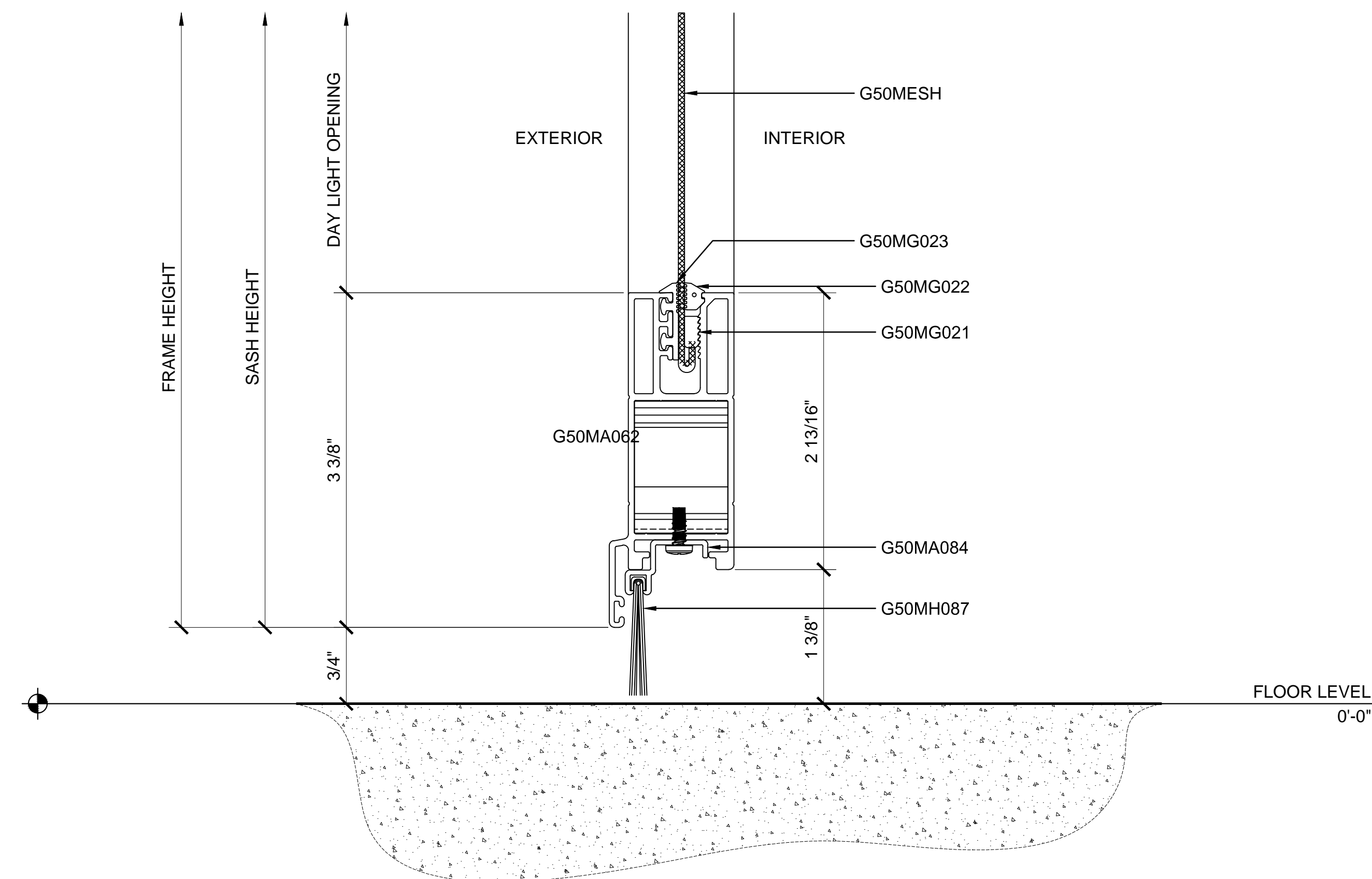
② SECTION DETAIL AT SILL
